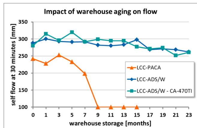
Fig. 7: Impact of warehouse aging of industrial packed castables on flow.
