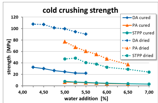
Fig. 3: Cured and dried cold crushing strength for test castables mixed with different water additions.
