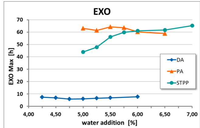
Fig. 2: EXO Max values for test castables mixed with different water additions.
